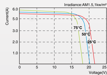
SLP090-12 I-V Curves
